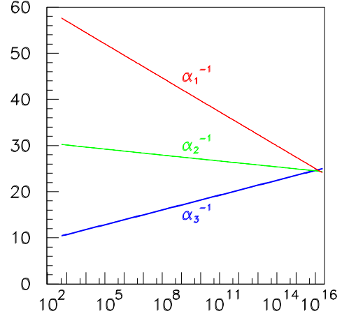
Figure 5: The measurements (vertical axis) of the gauge coupling strengths of the Standard Model at LEP and elsewhere can be evolved up to high energies (horizontal axis, in units of GeV) using renormalization-group equations incorporating supersymmetry. They are consistent with unification at a very high energy scale, but not with unification without supersymmetry [8].
